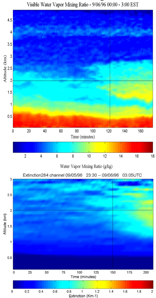
Figure 4. (a) Time sequences of water vapor profiles indicate the development of a cloud occurs before it is evident in the extinction profiles shown in (b); the lines are added to assist in locating corresponding points (Li et al. 2002, Philbrick et al 2005, Verghese et al. 2005).
