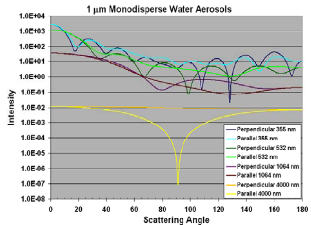
Figure 18. The scattering phase functions for 1 \mu\text{m} water aerosols are plotted for a 4- \lambda bistatic lidar.
